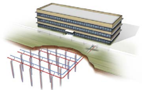
Figure 75. Vertical Bore Method
