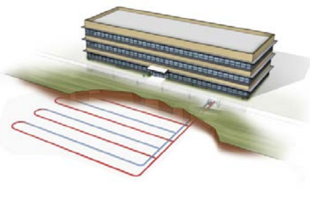
Figure 74. Horizontal Trench method
