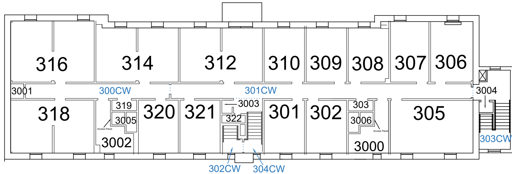
Third Floor Area 5753 S.F.
