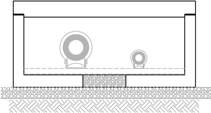
Figure 3 – Type B Tunnel Cross Section
