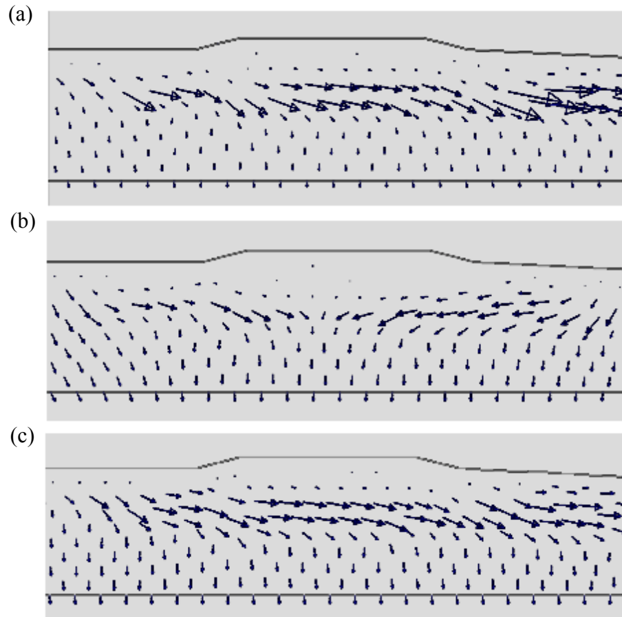
Figure 5-10. Comparison of flow vectors ( < 0.5 m/day) on day 42 of transect 3 model simulation for (a) calibrated model, (b) model with road as barrier, and (c) no road.
