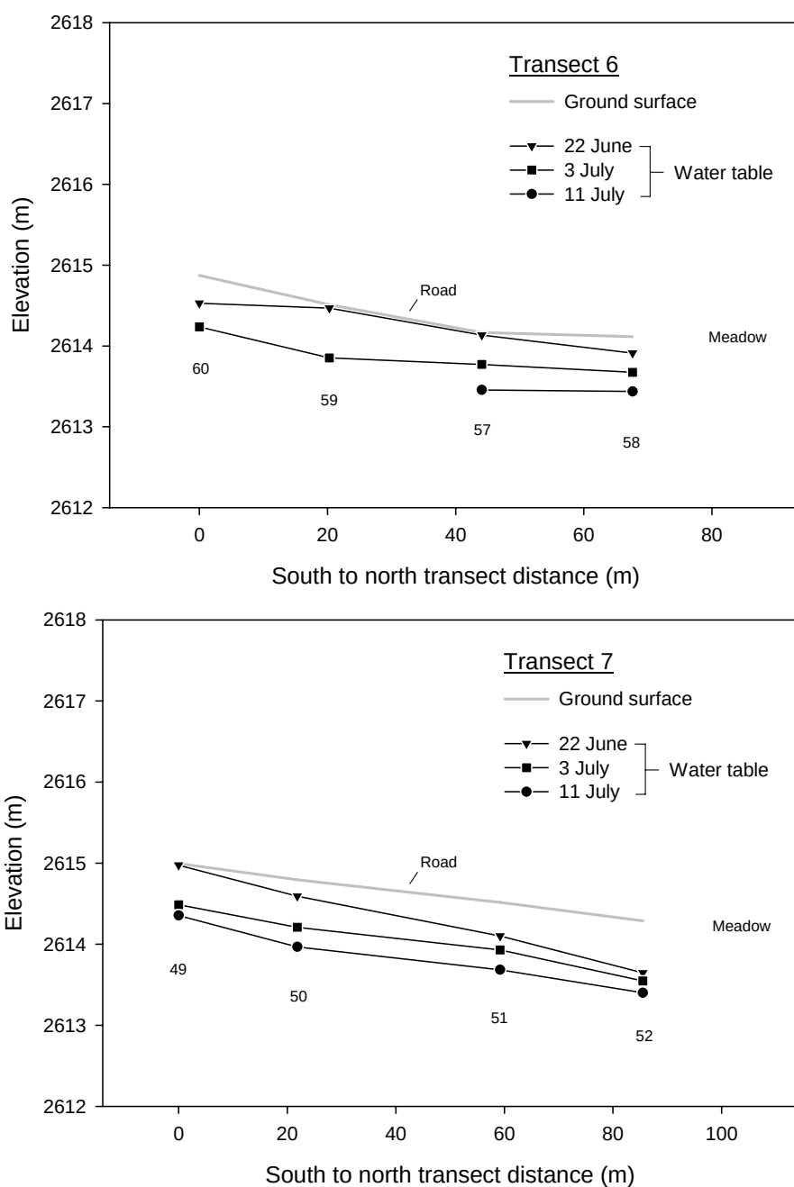
Figure 3-9. Ground surface and ground water levels along transects 6 (top) and 7 (bottom) for 22 June, 3 July and 11 July 2006. The location of the Tioga Road is identified by “road”.
