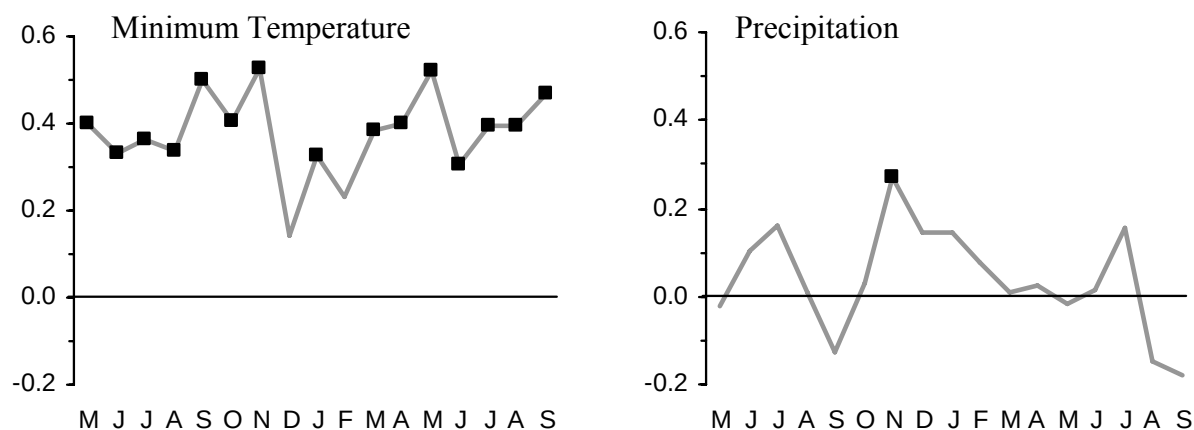
Figure 4-15. Correlation functions for the TFJ lodgepole pine standard tree-ring chronology. Black squares indicate significant correlations (99% confidence interval). The correlation functions examine monthly climate variables extending from May of the prior year to September of the current tree growth year.
