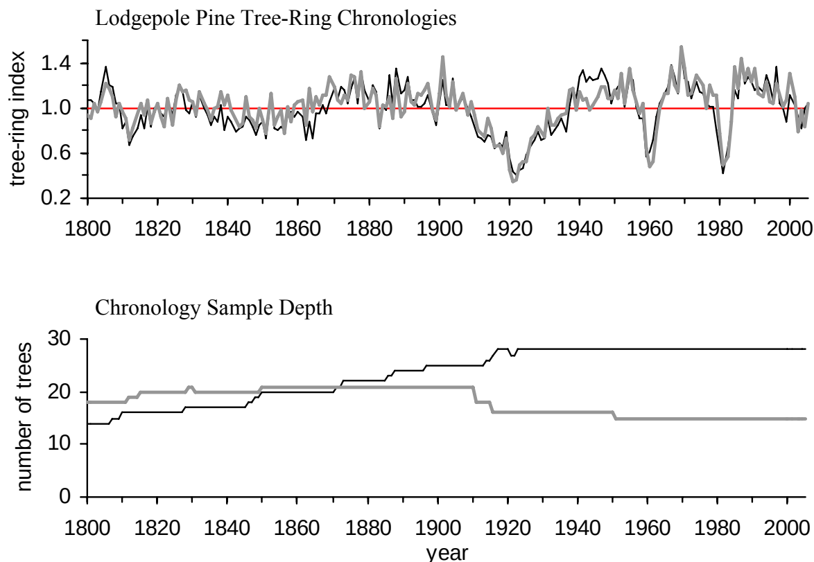
Figure 4-13. Standard tree-ring chronologies and chronology sample depth for Tioga Road trees (thin line) and TFJ trees (thick line). Sample depth reflects the number of trees incorporated into the chronology for each year of record.
